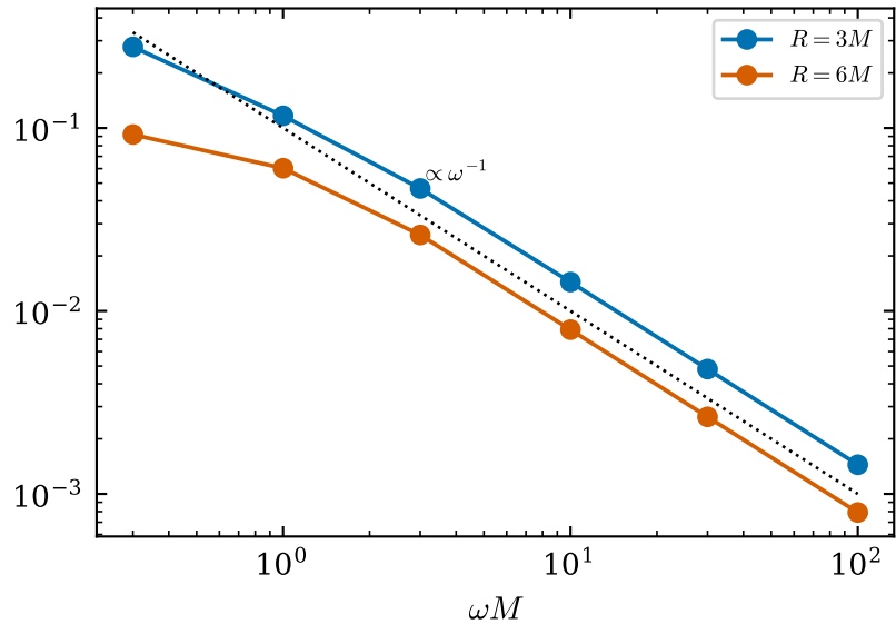
model A (frozen domain wall): constraint residual
