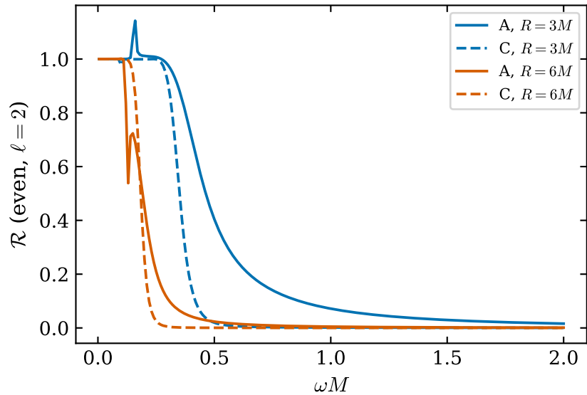
even parity: model A vs model C
